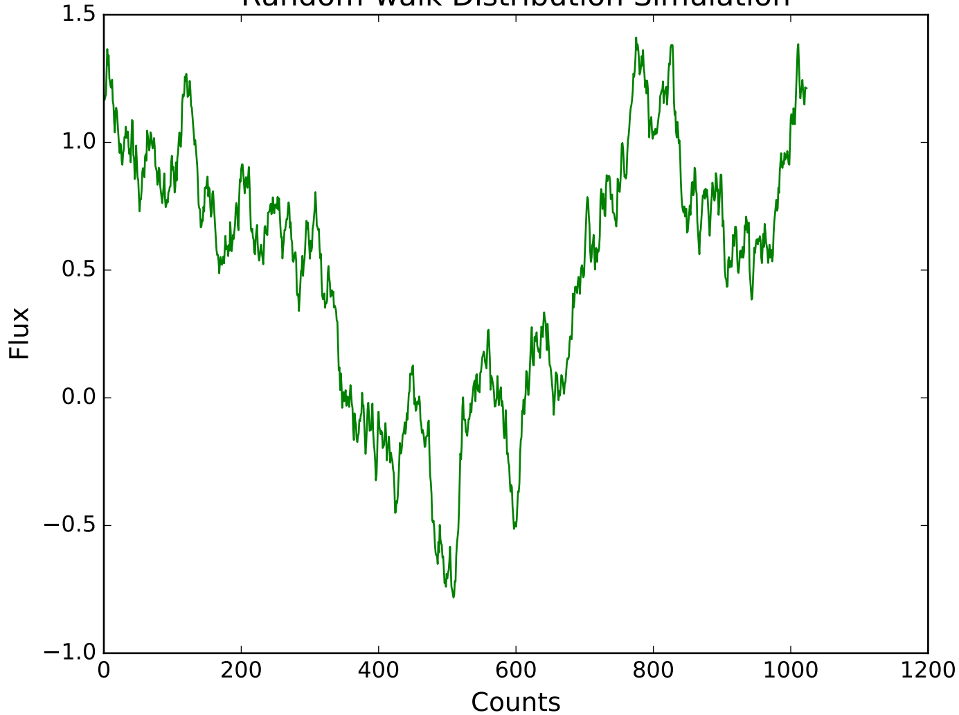
Random-walk Distribution Simulation
